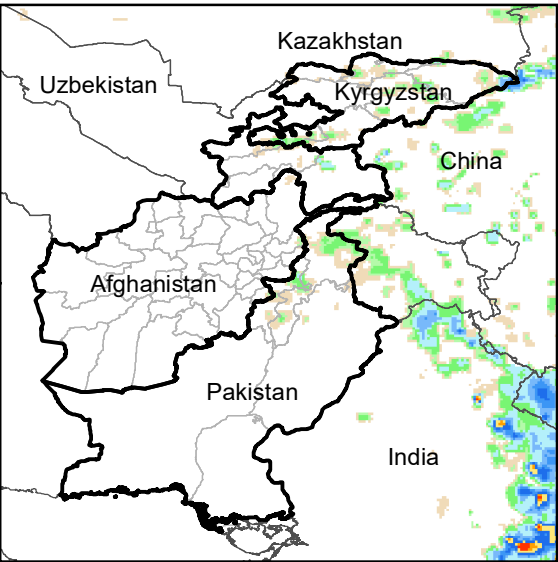
Daily Rainfall estimate for 11 Sep., 2002
