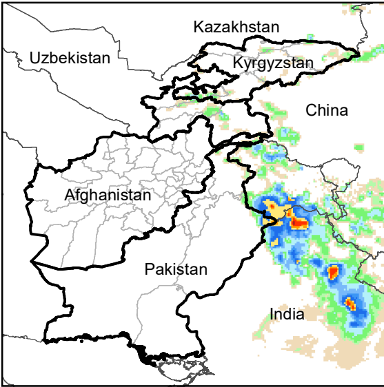
Daily Rainfall estimate for 13 Sep., 2002
