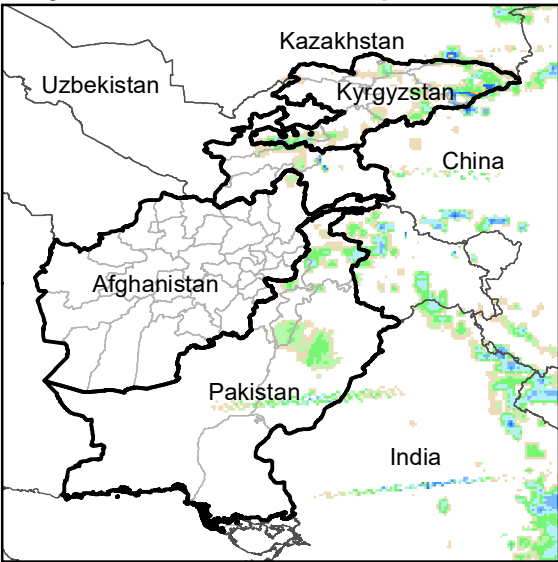
Daily Rainfall estimate for 12 Sep., 2002
