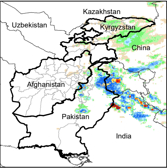
Daily Rainfall estimate for 17 Sep., 2002
