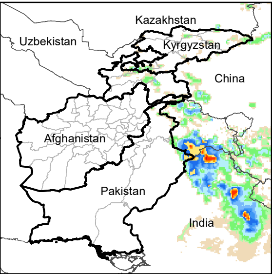
Daily Rainfall estimate for 16 Sep., 2002
