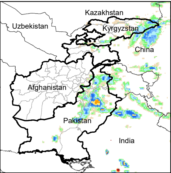
Daily Rainfall estimate for 21 Sep., 2002
