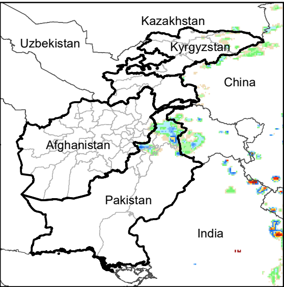
Daily Rainfall estimate for 26 Sep., 2002
