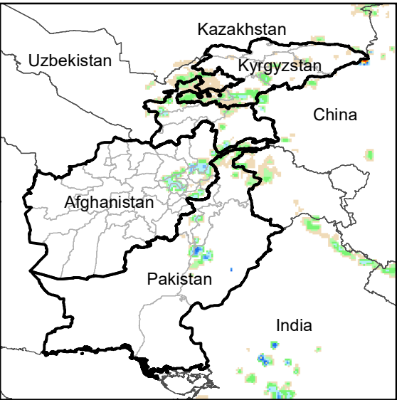
Daily Rainfall estimate for 29 Sep., 2002
