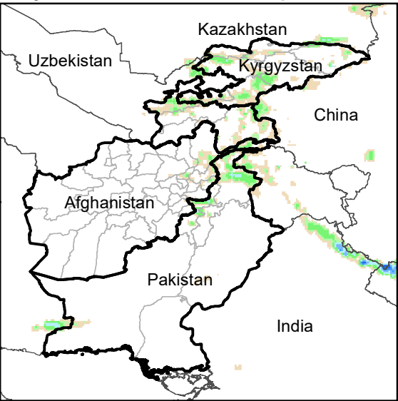
Daily Rainfall estimate for 30 Sep., 2002
