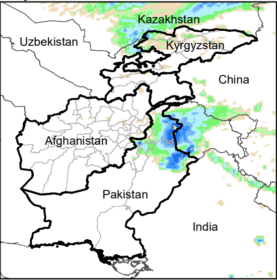
Daily Rainfall estimate for 13 Oct., 2002
