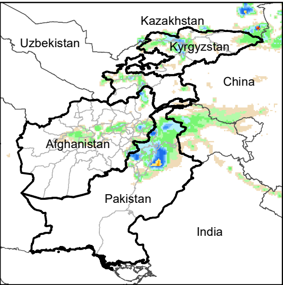
Daily Rainfall estimate for 23 Oct., 2002
