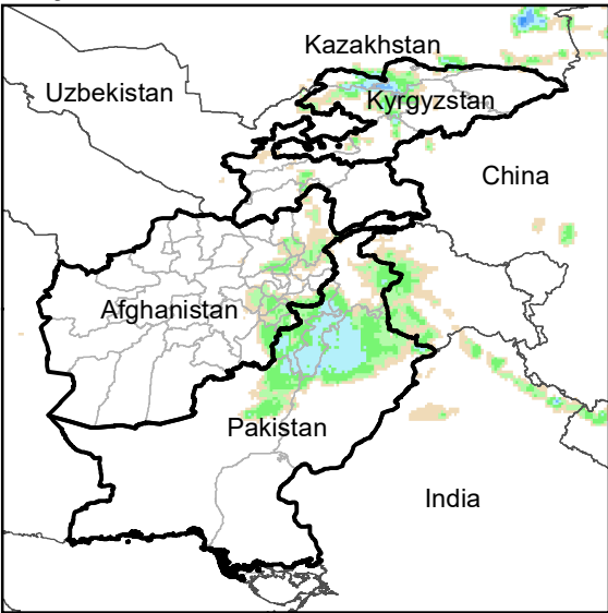
Daily Rainfall estimate for 24 Oct., 2002
