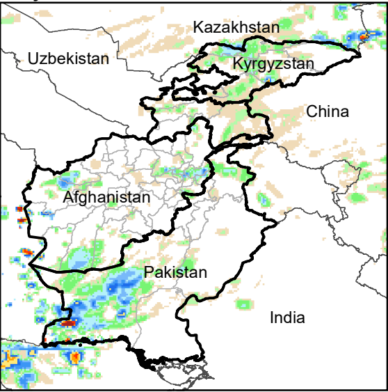
Daily Rainfall estimate for 8 Nov., 2002
