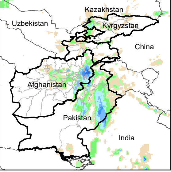
Daily Rainfall estimate for 11 Nov., 2002
