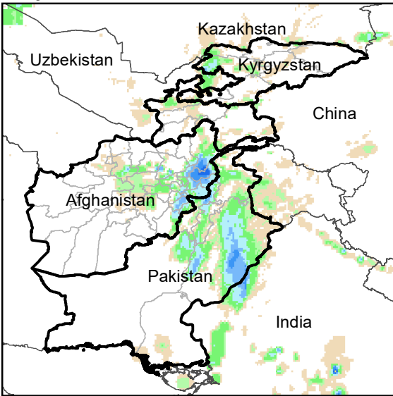
Daily Rainfall estimate for 14 Nov., 2002
