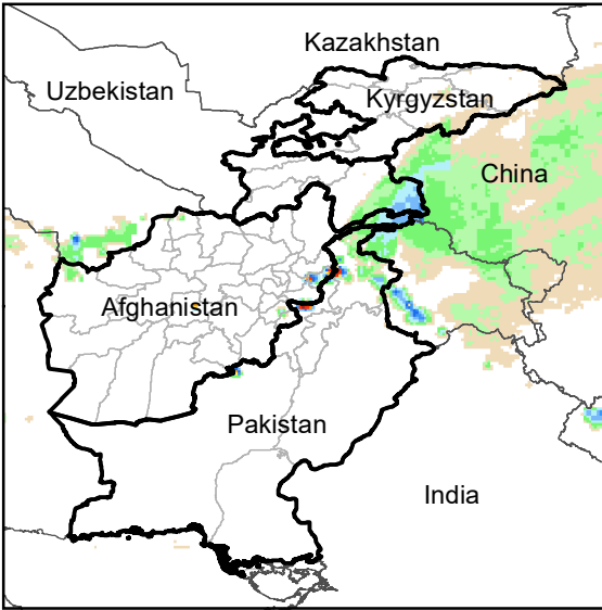
Daily Rainfall estimate for 5 Dec., 2002
