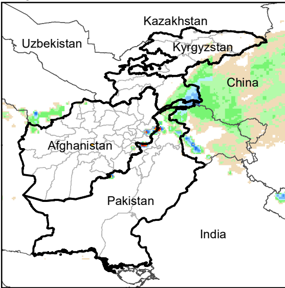
Daily Rainfall estimate for 8 Dec., 2002
