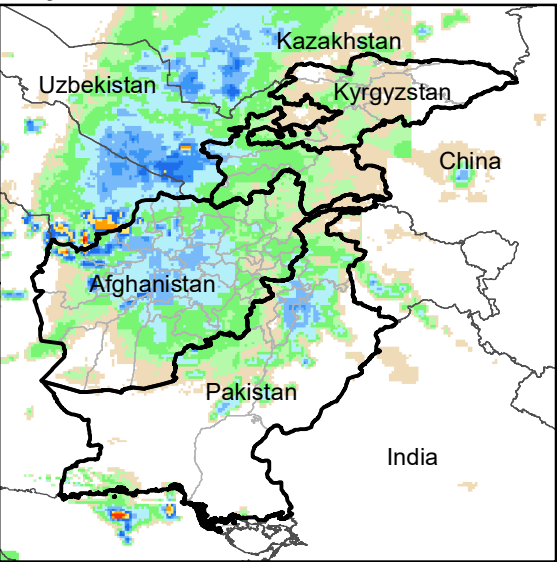
Daily Rainfall estimate for 26 Dec., 2002
