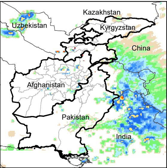
Daily Rainfall estimate for 3 Feb., 2003
