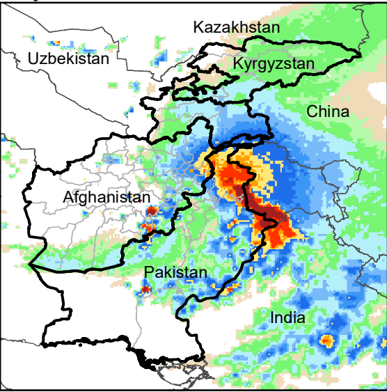
Daily Rainfall estimate for 18 Feb., 2003
