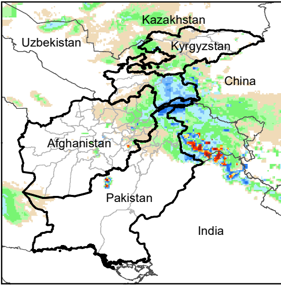
Daily Rainfall estimate for 20 Feb., 2003
