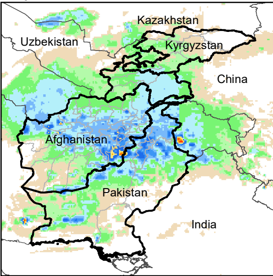
Daily Rainfall estimate for 19 Feb., 2003
