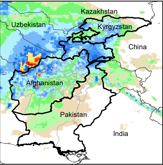
Daily Rainfall estimate for 14 Mar., 2003
