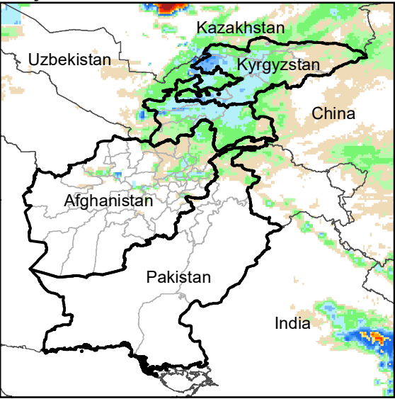
Daily Rainfall estimate for 19 Mar., 2003
