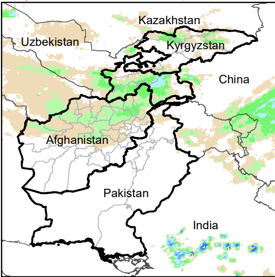
Daily Rainfall estimate for 8 Apr., 2003
