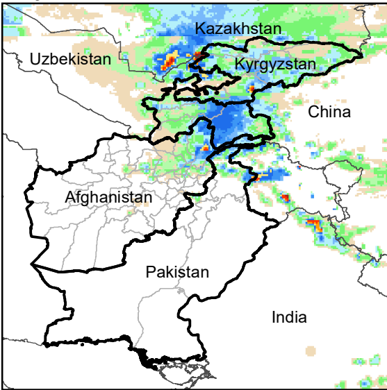
Daily Rainfall estimate for 9 Apr., 2003
