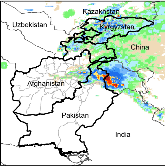
Daily Rainfall estimate for 1 May., 2003
