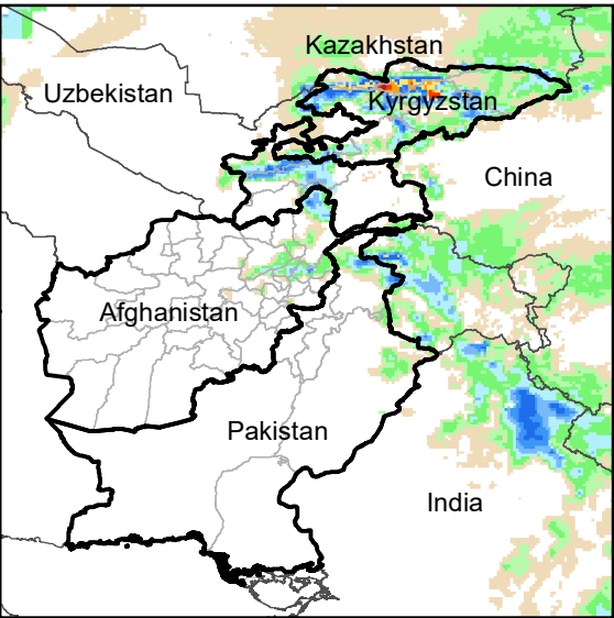
Daily Rainfall estimate for 30 Apr., 2003
