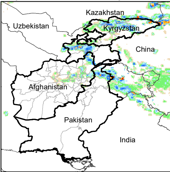
Daily Rainfall estimate for 9 May., 2003
