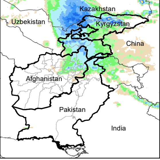
Daily Rainfall estimate for 10 May., 2003
