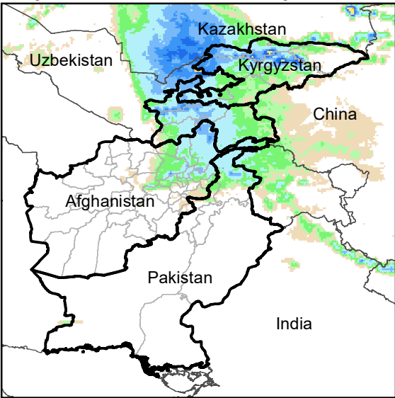
Daily Rainfall estimate for 13 May., 2003
