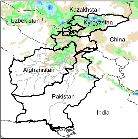
Daily Rainfall estimate for 14 May., 2003
