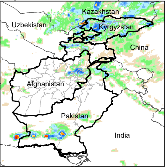
Daily Rainfall estimate for 29 May., 2003
