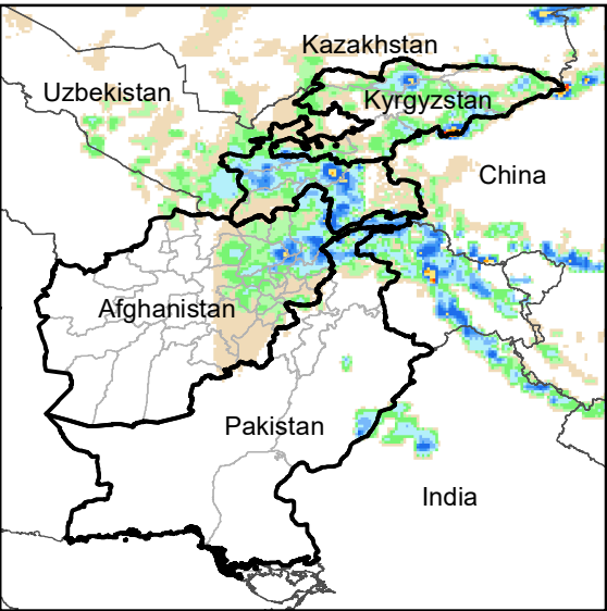
Daily Rainfall estimate for 3 Jun., 2003
