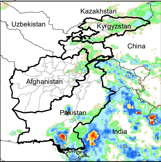
Daily Rainfall estimate for 18 Jun., 2003
