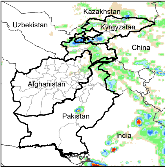
Daily Rainfall estimate for 20 Jun., 2003
