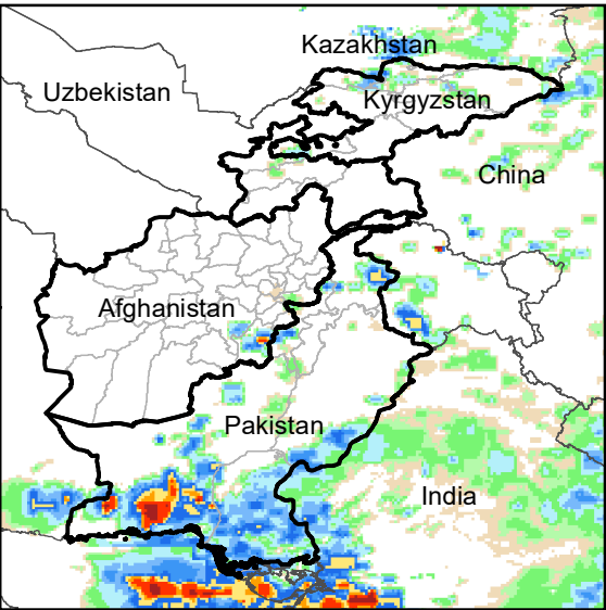
Daily Rainfall estimate for 11 Jul., 2003
