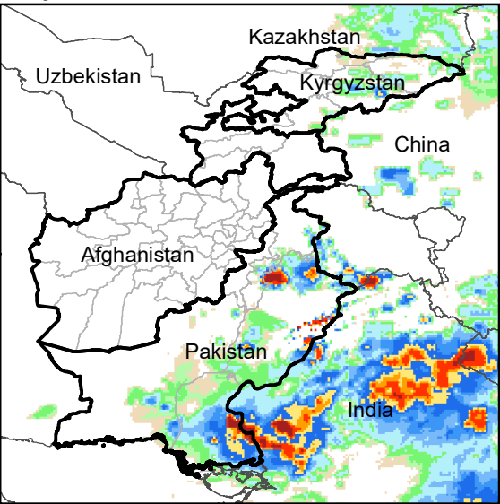
Daily Rainfall estimate for 13 Jul., 2003
