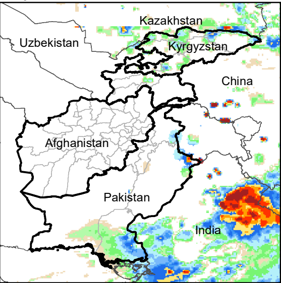
Daily Rainfall estimate for 14 Jul., 2003
