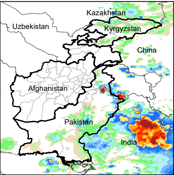
Daily Rainfall estimate for 12 Jul., 2003
