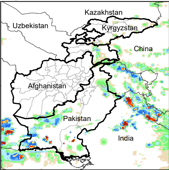
Daily Rainfall estimate for 2 Aug., 2003
