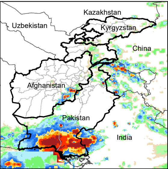
Daily Rainfall estimate for 1 Aug., 2003
