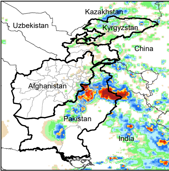
Daily Rainfall estimate for 3 Aug., 2003
