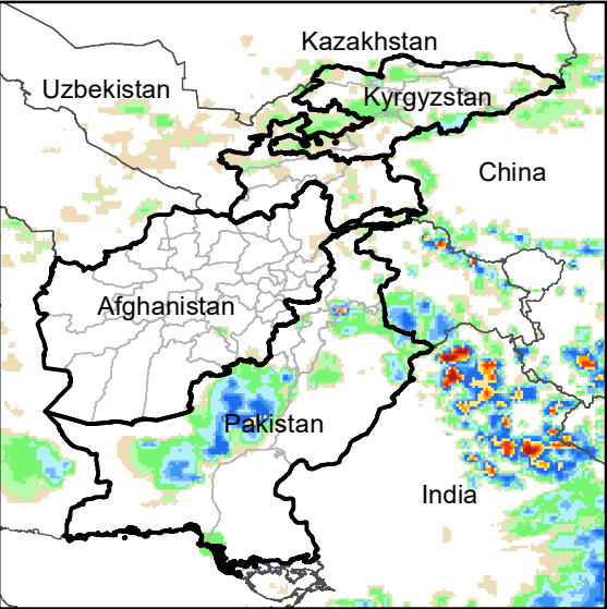
Daily Rainfall estimate for 4 Aug., 2003
