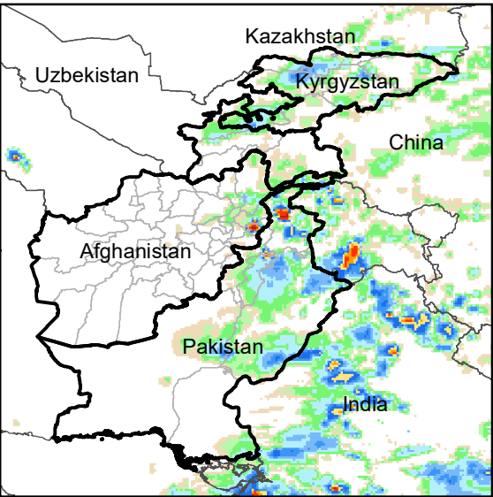
Daily Rainfall estimate for 7 Aug., 2003
