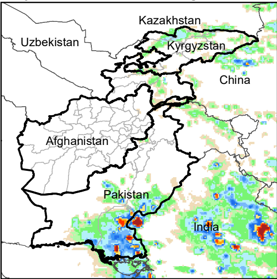
Daily Rainfall estimate for 9 Aug., 2003
