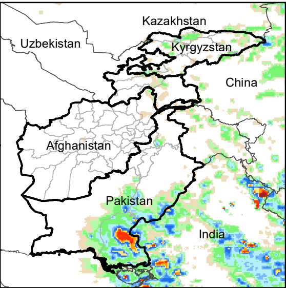
Daily Rainfall estimate for 8 Aug., 2003
