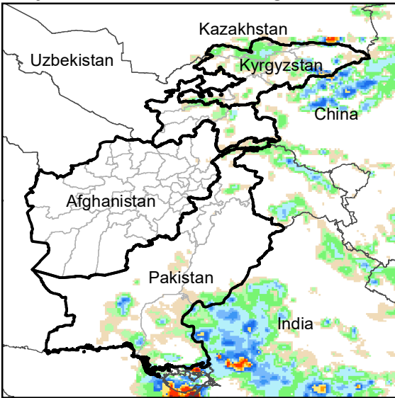
Daily Rainfall estimate for 10 Aug., 2003
