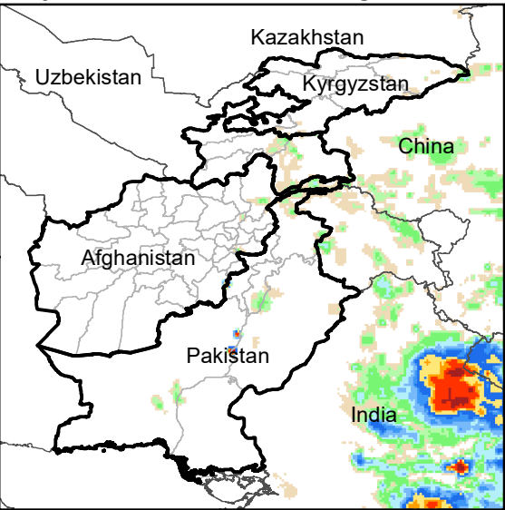
Daily Rainfall estimate for 17 Aug., 2003
