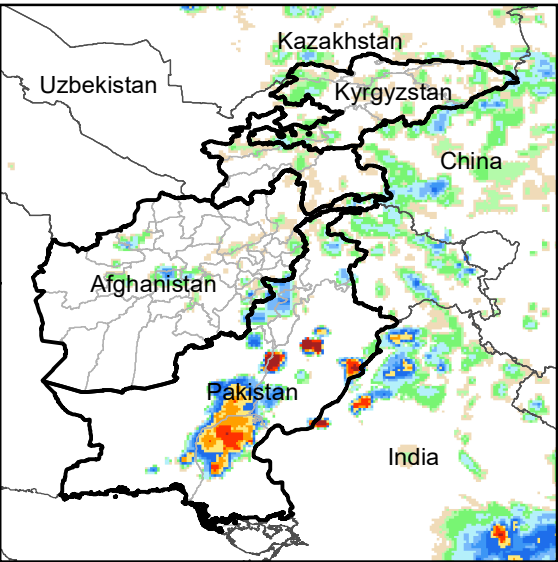
Daily Rainfall estimate for 24 Aug., 2003
