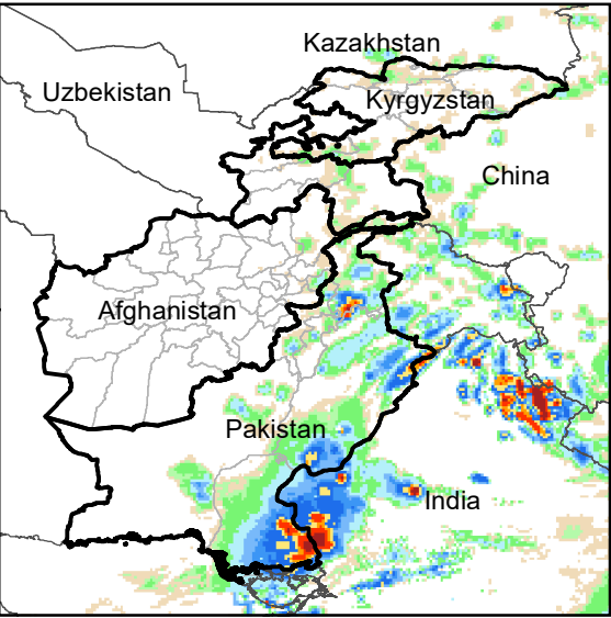
Daily Rainfall estimate for 26 Aug., 2003
