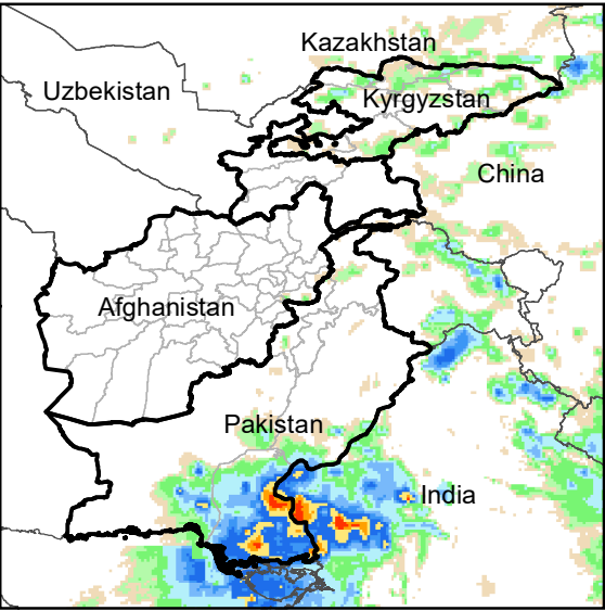
Daily Rainfall estimate for 25 Aug., 2003
