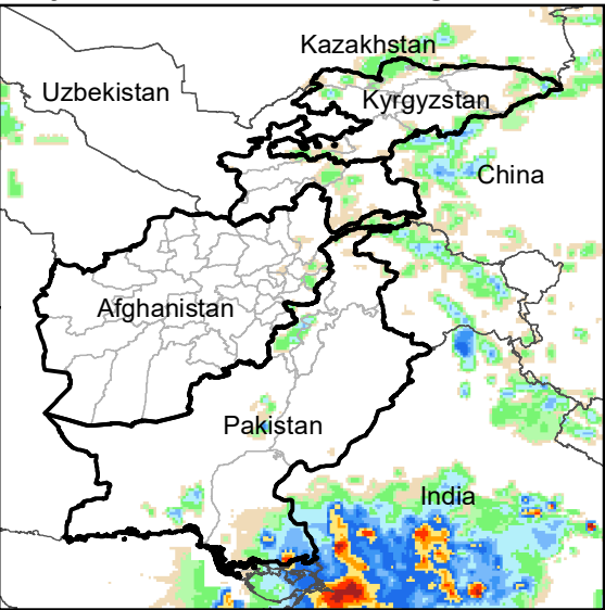
Daily Rainfall estimate for 27 Aug., 2003
