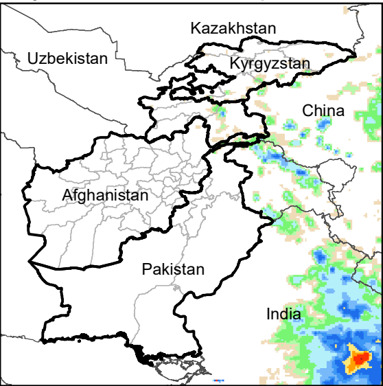
Daily Rainfall estimate for 4 Sep., 2003
