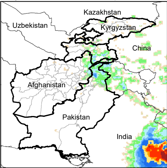
Daily Rainfall estimate for 11 Sep., 2003
