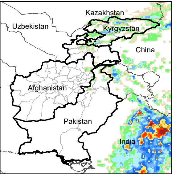
Daily Rainfall estimate for 18 Sep., 2003
