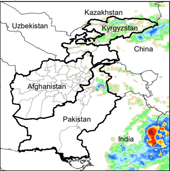
Daily Rainfall estimate for 19 Sep., 2003
