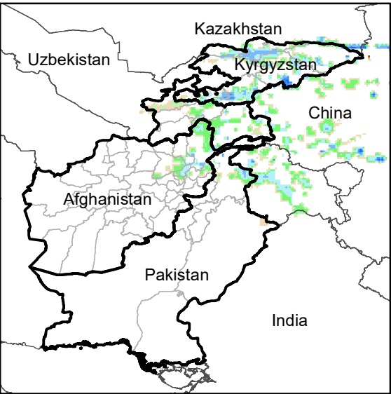
Daily Rainfall estimate for 13 Oct., 2003
