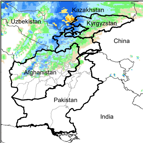
Daily Rainfall estimate for 4 Nov., 2003
