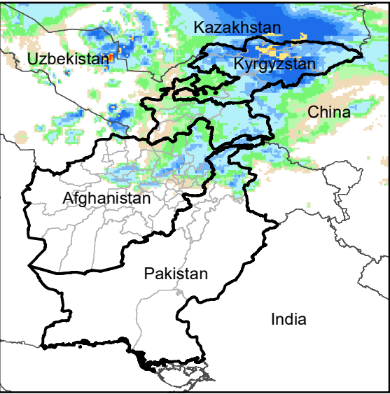
Daily Rainfall estimate for 5 Nov., 2003
