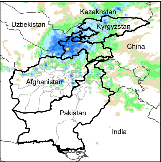
Daily Rainfall estimate for 19 Nov., 2003
