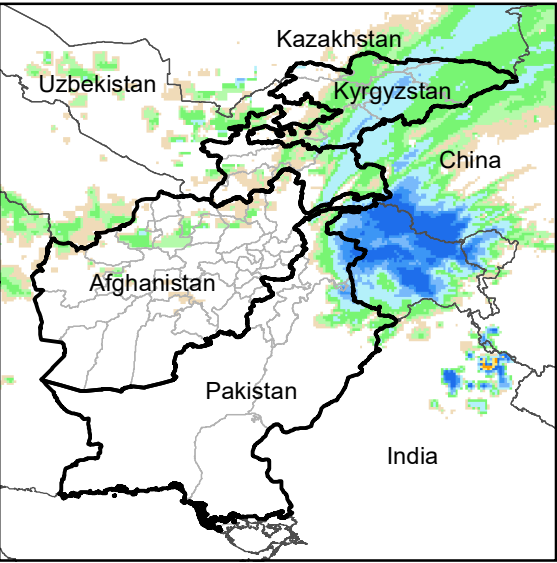
Daily Rainfall estimate for 13 Dec., 2003
