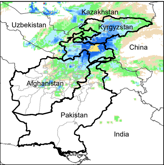
Daily Rainfall estimate for 11 Dec., 2003
