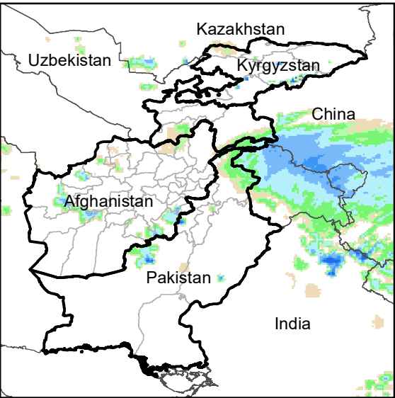
Daily Rainfall estimate for 3 Feb., 2004
