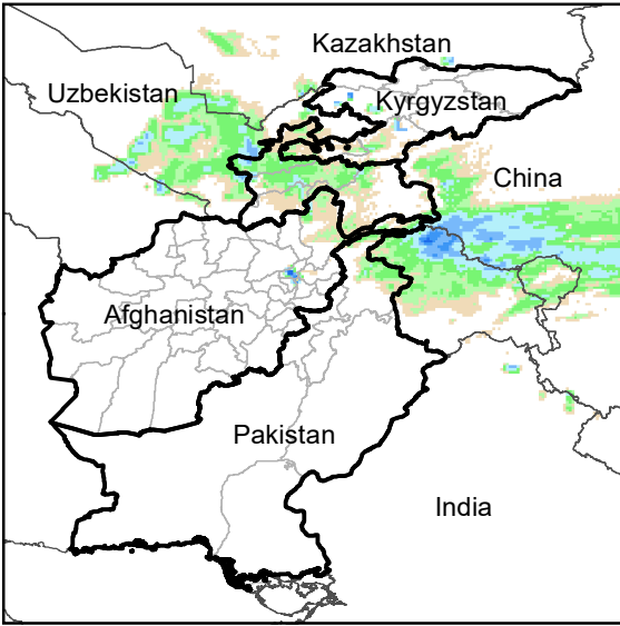
Daily Rainfall estimate for 29 Feb., 2004
