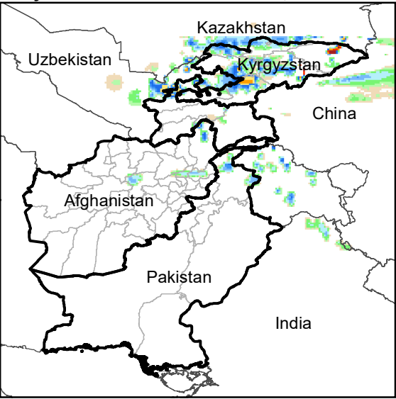
Daily Rainfall estimate for 9 Mar., 2004
