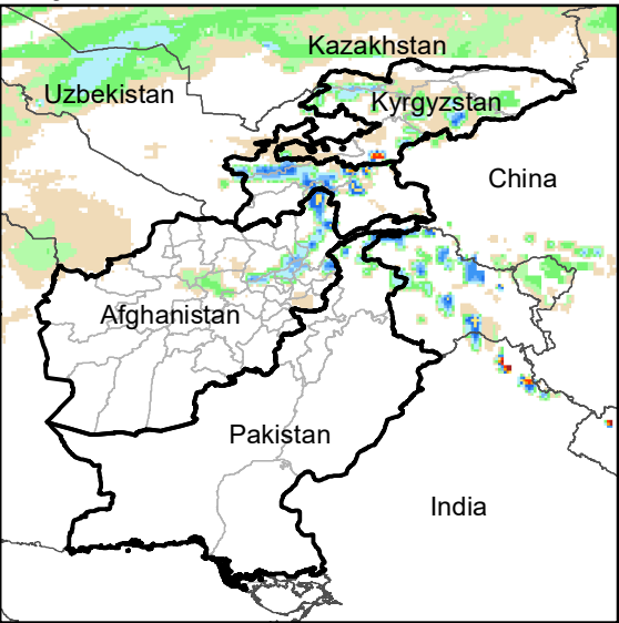
Daily Rainfall estimate for 10 Mar., 2004
