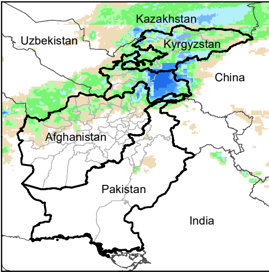
Daily Rainfall estimate for 13 Mar., 2004
