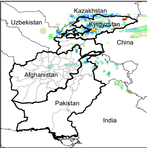
Daily Rainfall estimate for 12 Mar., 2004
