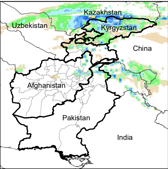
Daily Rainfall estimate for 11 Mar., 2004
