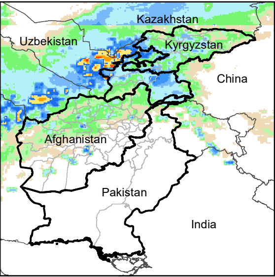
Daily Rainfall estimate for 15 Mar., 2004
