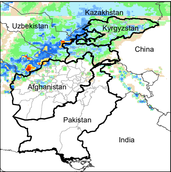
Daily Rainfall estimate for 19 Mar., 2004
