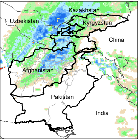
Daily Rainfall estimate for 9 Apr., 2004
